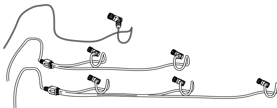
RSSE0017 cable replacement ERA200 2x18 AWG for one-light module RSSE0017 cable replacement ERA200 3x18 AWG for two-light module RSSE0017 cable replacement ERA200 4x18 AWG for three-light module
